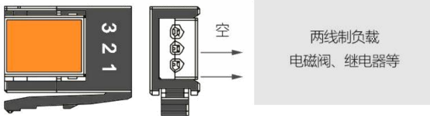
E-CON连接器公端子3Pin
